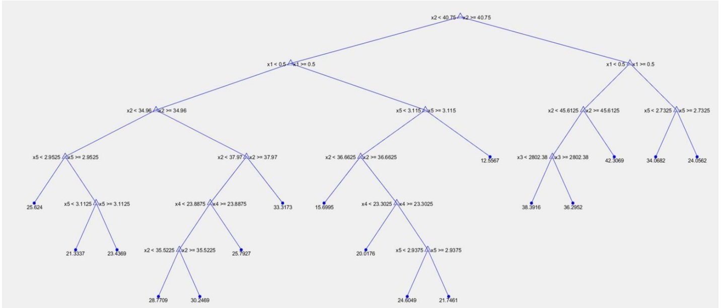
Figure 1 Regression Tree Analysis, X2 = Abdomen Circumference
